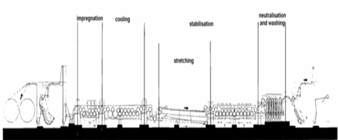
Fig.7 Diagram Showing Chainless Mercerization
