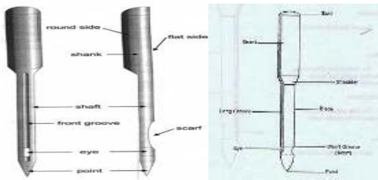
Fig 2.6.1 part of sewing machine needle
